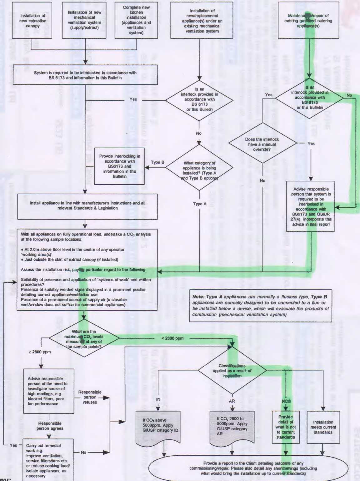
Figure 1 - Flowchart dealing with assessment protocol when dealing with gas-fired commercial catering appliances
